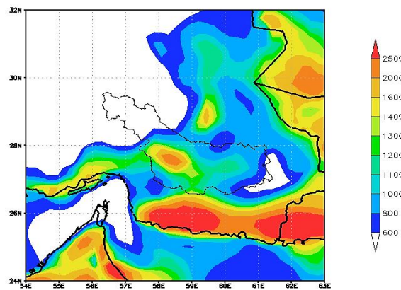
Fig. 4. Surface concentration values of WRF_Chem model output particles at UTC18 on December 17, 2016.
