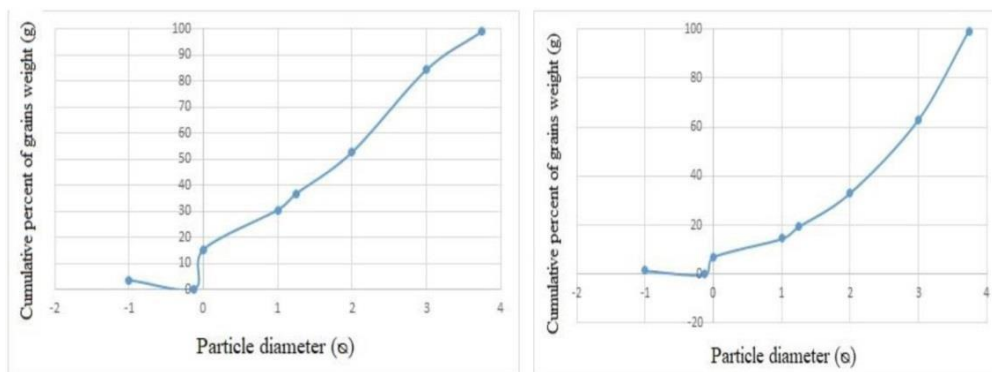
Fig. 5. Accumulative grain size plot; left: sample of control reach, right: sample of backwater reach
